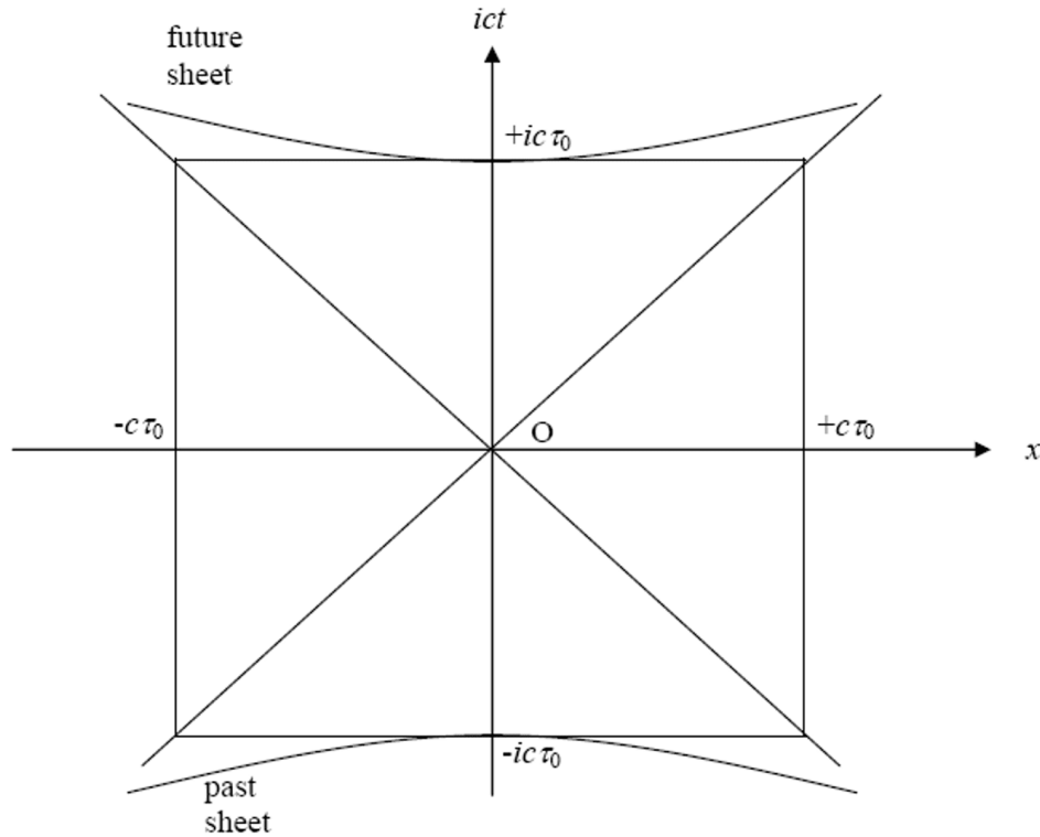
Figure 2. Castelnovo spacetime, with its light-cone and its de Sitter horizon. O is the tangency point on spacetime.
