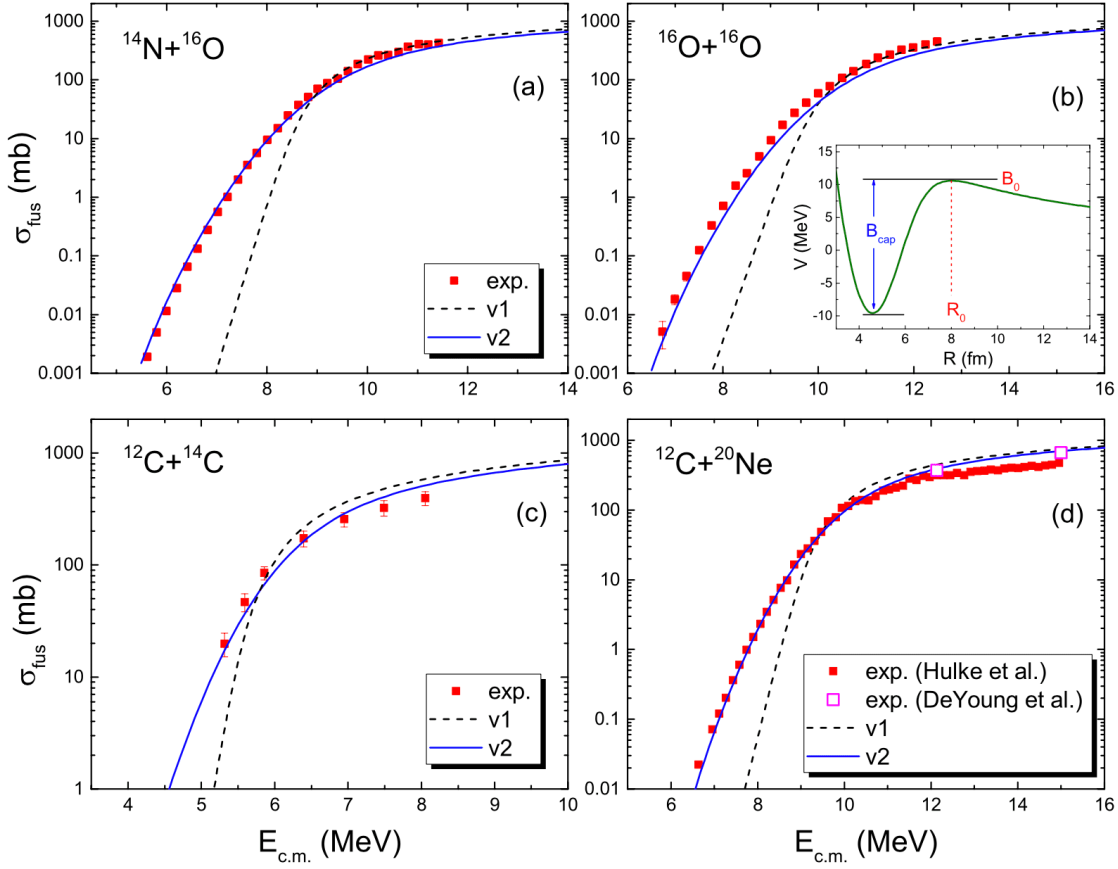
Figure 1. Fusion excitation functions for reactions ^{14}\text{N} + ^{16}\text{O} [42] , ^{16}\text{O} + ^{16}\text{O} [43] , ^{12}\text{C} + ^{14}\text{C} [44] and ^{12}\text{C} + ^{20}\text{Ne} [45] [46] . Sub-figure: Entrance channel nucleus-nucleus potential for ^{16}\text{O} + ^{16}\text{O} . The red dashed line in the sub-figure denotes the position of the barrier radius R_0 and the blue line denotes the depth of the capture pocket B_{\text{cap}} .
