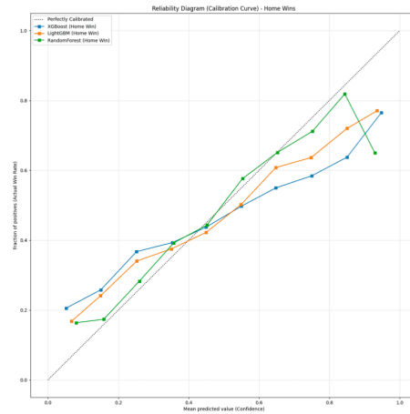
(b) Calibration Curve
