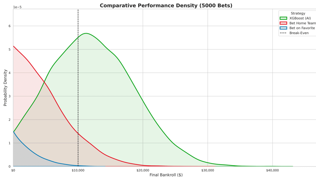
Figure 7. Comparative Performance Density. This chart overlays the AI’s performance (green) against human strategies. The AI curve is taller and shifted right, meaning it produces consistent, moderate results more often than the volatile human strategies.
