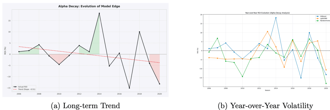
Figure 2. Alpha Decay Analysis. (a) The stylized trend showing the "Golden Age" (green) vs the "Efficient Era" (red). (b) The raw performance lines for all three models, showing the specific volatility and the sharp drop-off for XGBoost (blue) after 2014.
