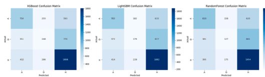
(a) Confusion Matrices
