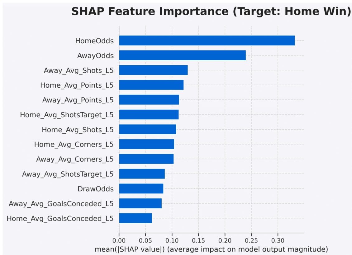
Figure 5. SHAP Feature Importance. The blue bars represent how much each data point contributed to the AI’s decision. The most important feature was “HomeOdds”—the price set by the bookmaker. This suggests the AI spent more effort analyzing the market price than the actual team statistics (like Shots or Points).
