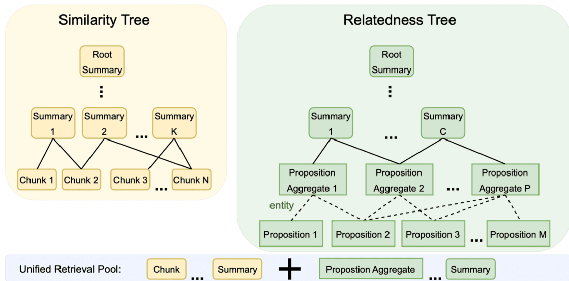
Figure 2. SiReRAG Tree. We adopt RAPTOR [4] to construct the similarity tree (left). On the right, we construct the relatedness tree by clustering the propositions based on their entities to get proposition aggregates and having recursive summaries on top. Note that propositions are not included in the relatedness tree, so their connections to proposition aggregates are marked with dashed lines.
