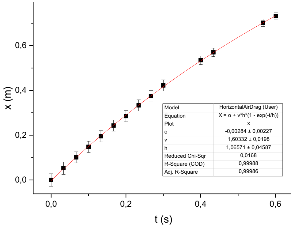
Figure C29 – X-axis, motion plot with air resistance
