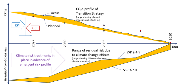
Figure 3. Example of a measurable climate risk and decarbonization transition strategy. The CO 2 e profile above the horizontal axis shows stage objectives (red diamonds) with idealized and sequenced decarbonization profiles; the key performance indicators and key risk indicators are aligned by the objective to provide 360° reporting. The residual risk profiles for two climate change scenarios are shown against the stage objectives below the horizontal axis. Substantive and transparent business transitions can be measured and independently verified. Reproduced by the kind permission of Southern Harbour Ltd.
