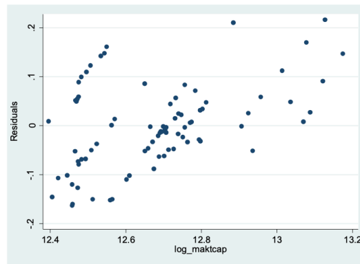
Graph 1. Residuals plot against the predicted values (log_maktcap)
