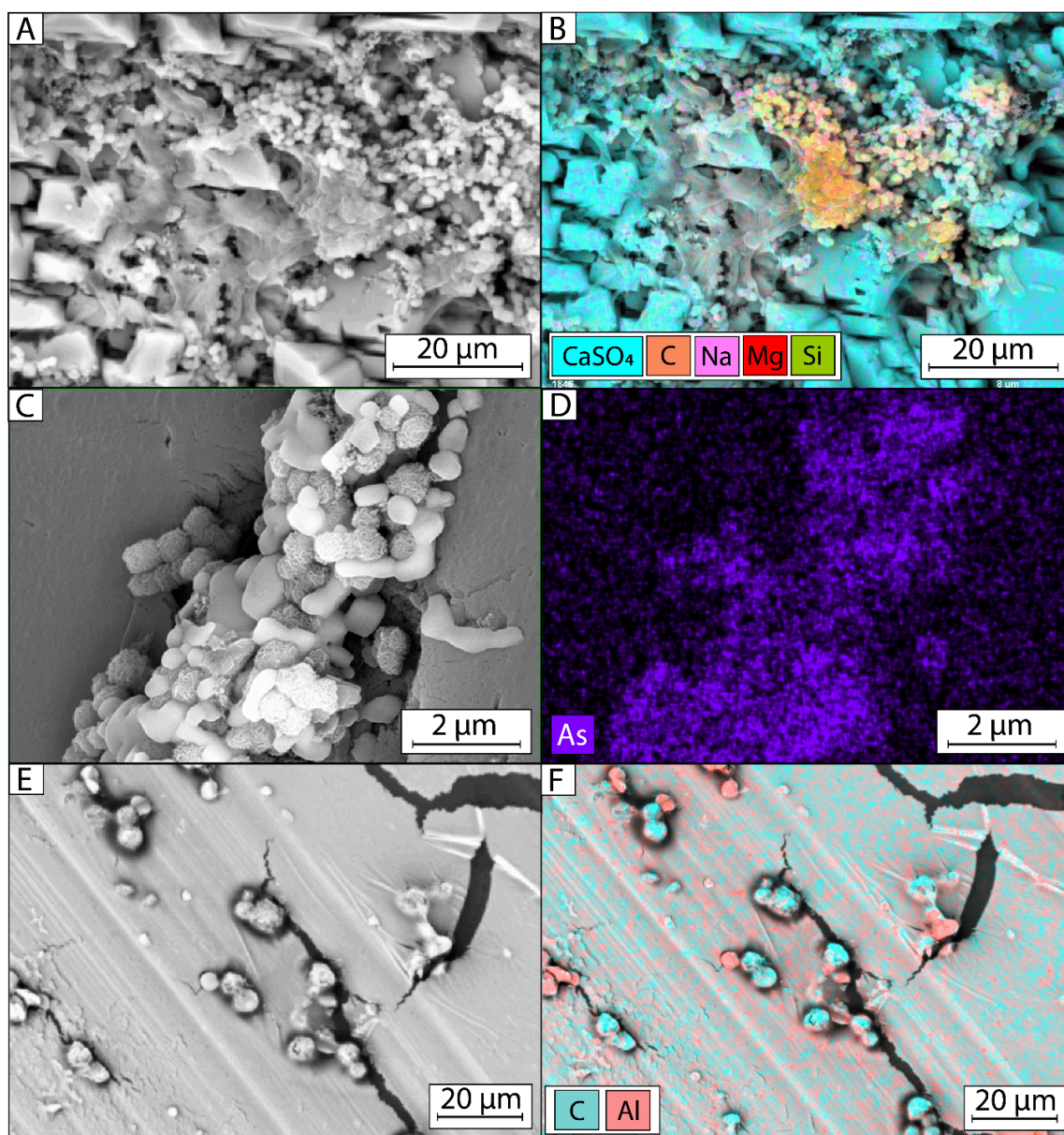
Figure 8. SEM microphotographs (A, C, E) and EDS mapping (B, D, F) of PAJ (A-B-C-D) and GOR (E-F) gypsum samples. (A) EPS-embedded crystals and Mg-Si globules on heavily altered gypsum surface. (B) Mg-Si and Na are concentrated below the biomass, suggesting both Mg-Si globules and Na-Ca sulfates are agglutinated. (C) Porosity filled with allotriomorphic halite and Mg-Si globules. (D) Globules appear to be also As-rich according to EDS mapping. (E) Twinned lenticular aggregates covering GOR gypsum surface. (F) EDS mapping shows that they are rich in K, Al and S, suggesting alunite.
