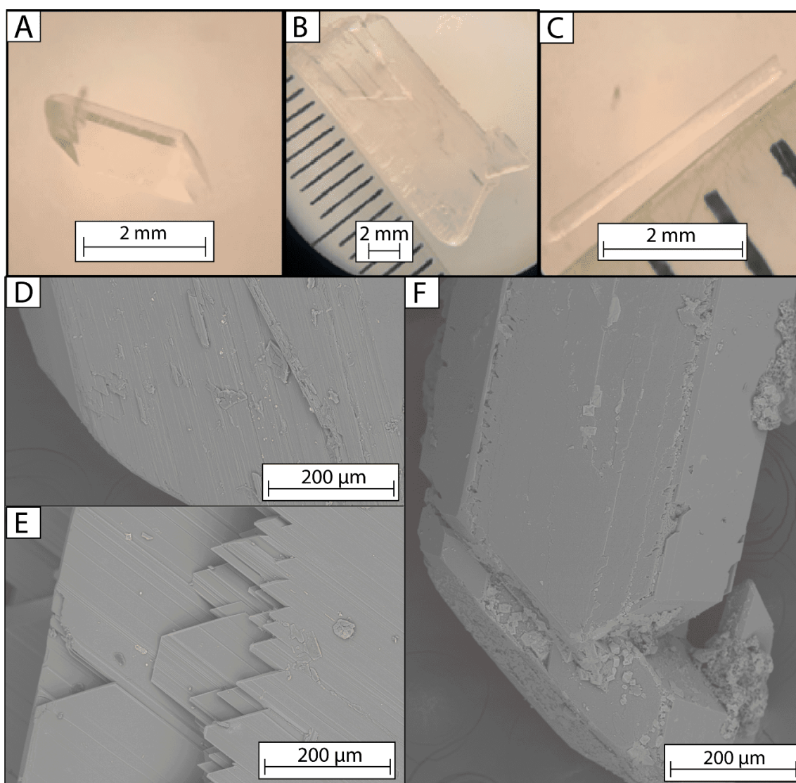
Figure 3. Gypsum crystal morphologies observed in each salt flat brine under binocular lenses (A-C) and microphotographs captured via SEM (D-F). (A) Prismatic LLA gypsum crystal without exposed cleavage planes and no apparent twinning. (B) Tabular PAJ gypsum crystal with exposed cleavage planes and characteristic fishtail twinning. (C) Acicular GOR gypsum crystal with characteristic elongated C axis. (D) Well-developed prismatic LLA crystal with no signs of dissolution. (E) Tabular PAJ crystal displaying cleavage planes, fishtail twinning and no dissolution. (F) Twinned acicular GOR crystal and occasional halite aggregates atop.
