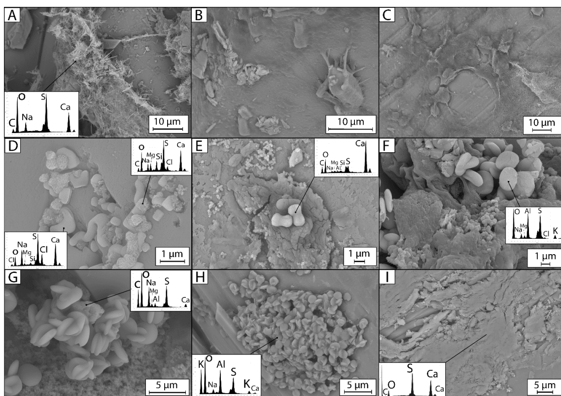
Figure 7. SEM microphotographs of LLA (A-C), PAJ (D-F) and GOR (G-I) gypsum crystals at 0 (first column), 35 (second column) and 90 days of experiments (third column). (A) Fibrous Na-Ca sulfate within and on top the alveolar EPS partially covering the LLA gypsum surface. (B) Thicker EPS layer embedding newly formed gypsum crystals. (C) Alveolar EPS embedding cells, fibrous Na-Ca sulfates and gypsum, and forming globular structures. (D) Mg-Silicate rugose globules and allotriomorphic halite filling porosities in PAJ gypsum. (E) Dumbbell-shaped calcite along with Mg-Si globules on the EPS. (F) Alveolar EPS-covered gypsum with Mg-Si globules and twinned lenticular K-Al sulfate on top. (G) Twinned lenticular K-Al sulfates with smooth surfaces with traces of C on a GOR gypsum crystal. (H) Lenticular crystal aggregates with jagged edges partially covering the gypsum surface, with scarce newly formed gypsum crystals. (I) Heavily altered gypsum surface with traces of carbon indicating organic matter.
