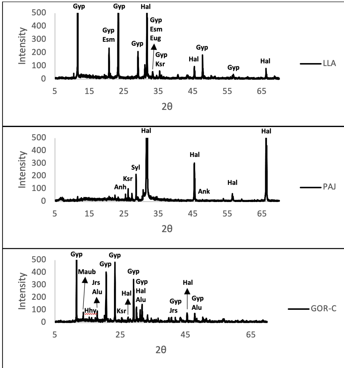
Figure S1. X-ray diffraction (XRD) patterns displaying intensity versus the diffractin angle ( 2\theta ) for LLA, PAJ and GOR-C samples. Mineral abbreviations: Gyp: gypsum, Hal: halite, Esm: epsomite, Syl: sylvite, Anh: anhydrite, Ksr: kieserite, Eug: eugsterite, Maub: magnesioaubertite, Alu: alunite, Jrs: jarosite, Hhy: hexahydrite, Ank: ankerite.
