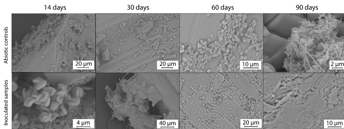
Figure S4. Time series of GOR gypsum crystals displaying the main textures and minerals found in each monitoring step in abiotic controls (first row) and inoculated samples (second row).
