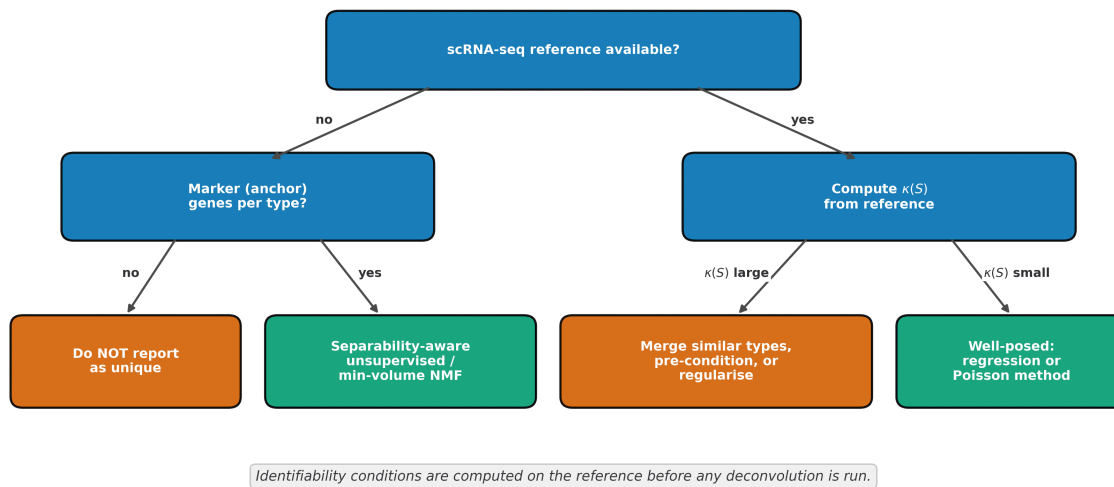
Figure 4. Identifiability-based algorithm selection for spatial-transcriptomics deconvolution
