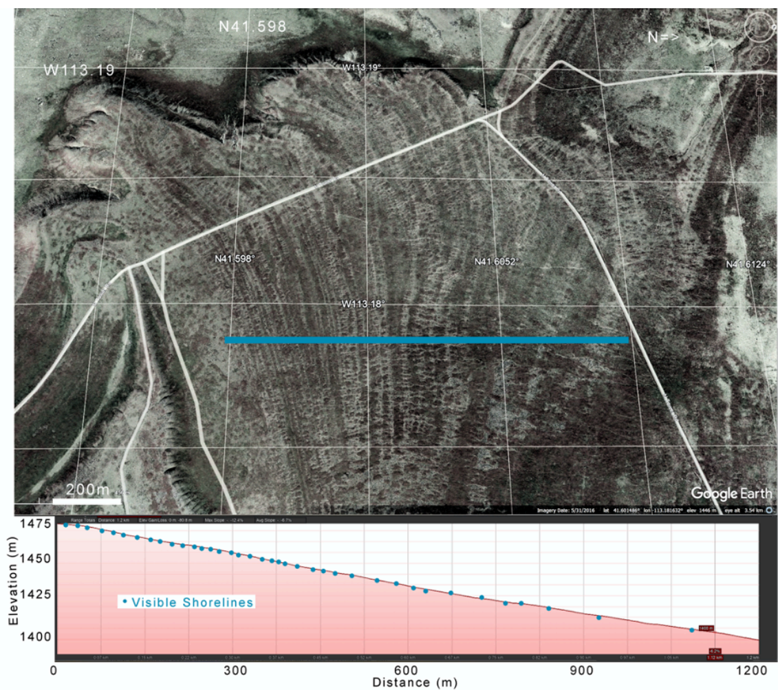
Figure 28. Google Earth™ view of bars on the north side of the Hogup Mountains from the fall from the Provo level. The bars are formed in expanding intervals in spite of the fact that the slope in this area is constant. The bars appear to be dependent on weight of lake removed and are thought to be resulting from IRPS. (41°36'N, 113°11'W)
