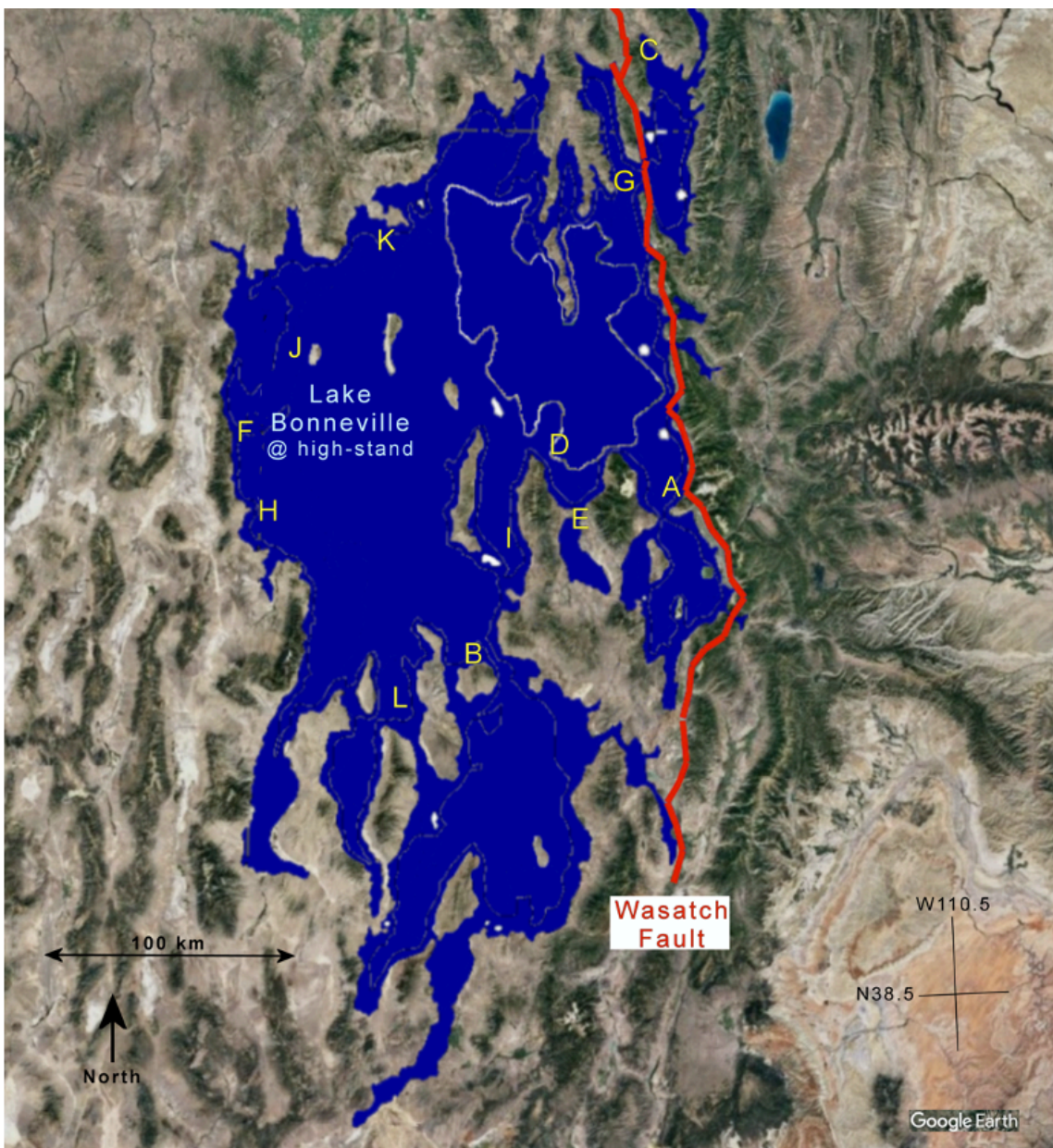
Figure 1. Lake Bonneville and the Wasatch Fault.
