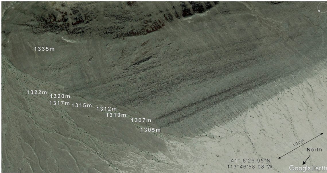
Figure 17. Google Earth™ view of cross-shore current surge deposits in the Pilot Valley attributed to the S30-Hansel-1335 Event surge. The calcium deposits at the top of the slope are the from waves crashing on the shore at the end of the event when there was a high concentration of stirred up calcium in the lake. The ascending double bands are from waves and secondary surges in each cycle of the event. (41°6'27"N, 113°46'58"W)
