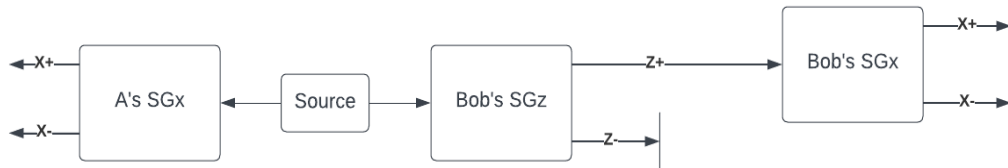
Figure 6 – A diagram of an experiment used to show when entanglement is broken.
