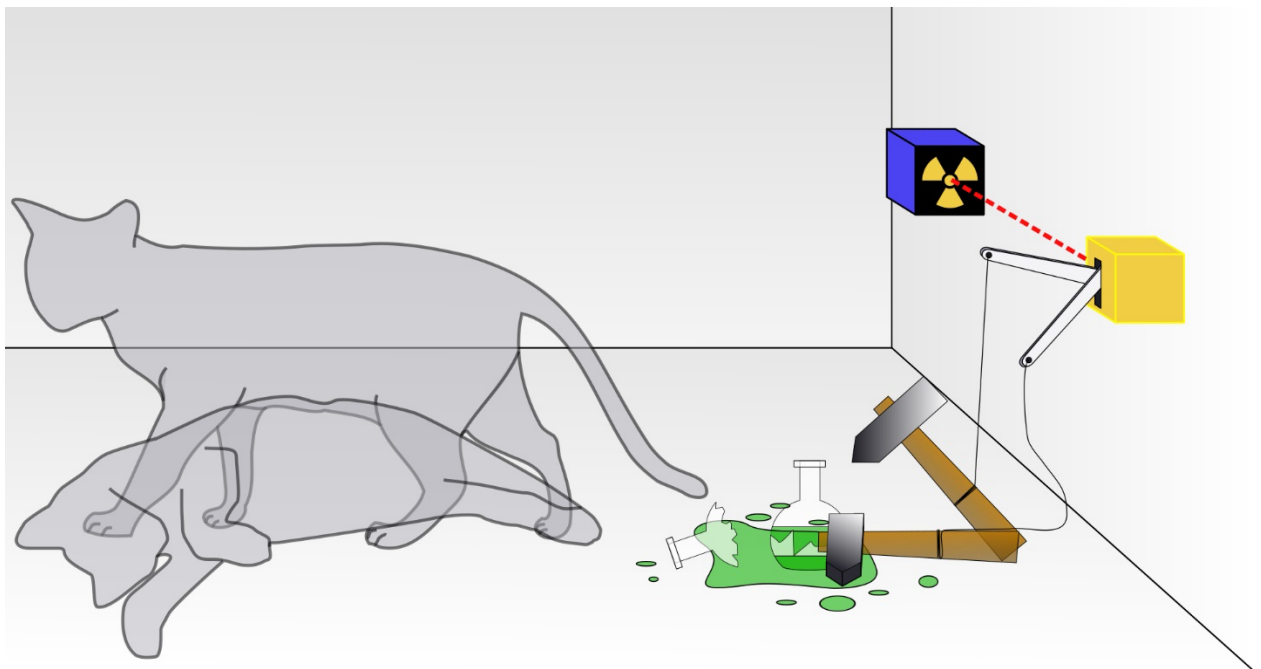
Figure 4 – Schrödinger’s cat.
