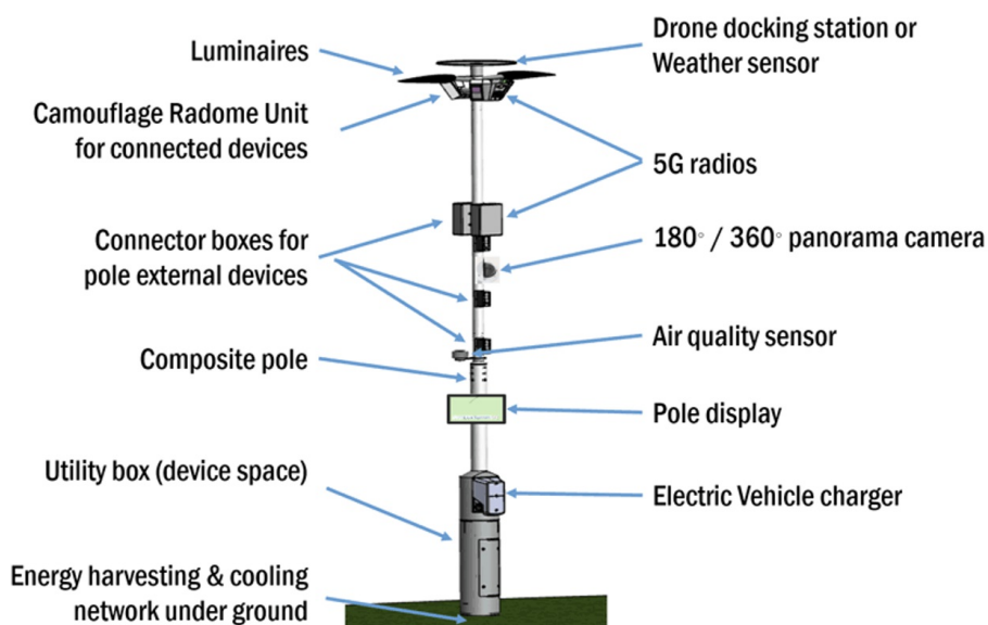
Figure 4. LuxTurrim5G light pole with integrated components of smart features- sensors and cameras (Source: https://ercim-news.ercim.eu/en117/special/luxturrim5g-smart-5g-light-pole-infrastructure-for-digital-service-ecosystems-in-cities )
