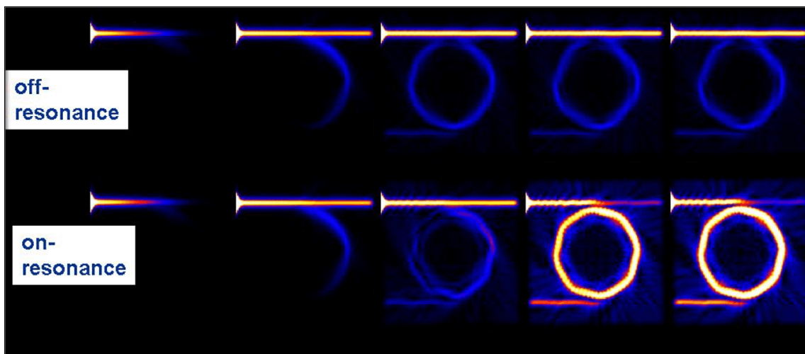
Figure 2b. Evolution of the numerical solution of the Helmholtz Equation for a microresonator being off- and on-resonance [25].
