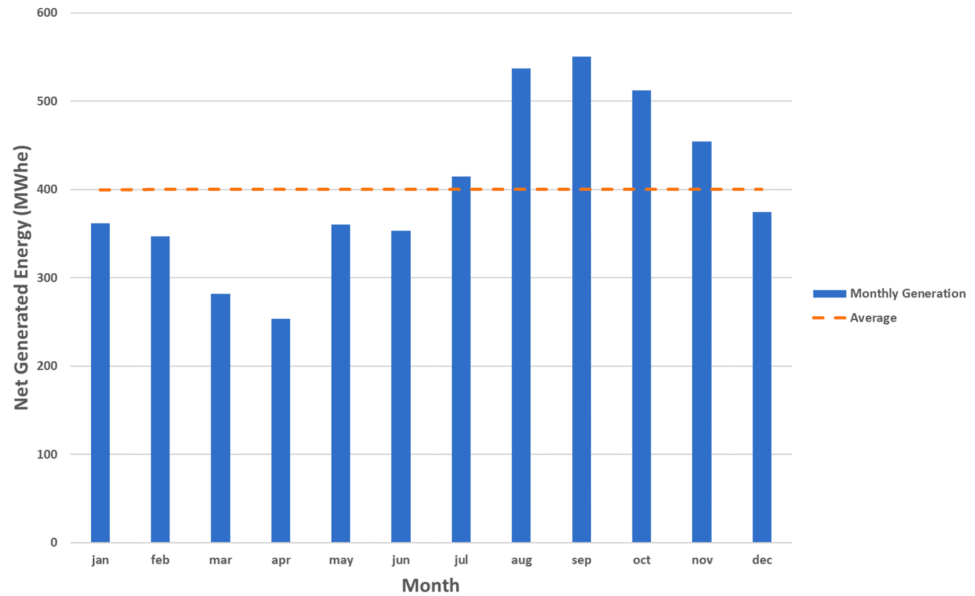
Figure 5. Monthly power generation for the optimum configuration.
