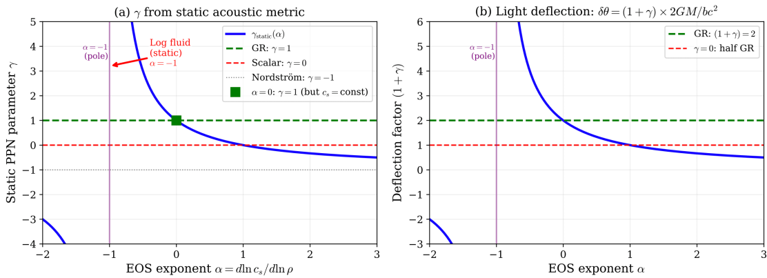
Figure 3. (a) Static PPN parameter \gamma(\alpha) = (1 - \alpha)/(1 + \alpha) . The logarithmic fluid at \bar{\rho} = \rho_\infty has \alpha = -1 , a pole of \gamma_{static} : the static acoustic metric is ill-defined. GR's \gamma = 1 is attained at \alpha = 0 , but this corresponds to density-independent c_s , which produces zero refractive deflection. (b) The same pathology in the deflection factor (1 + \gamma) .
