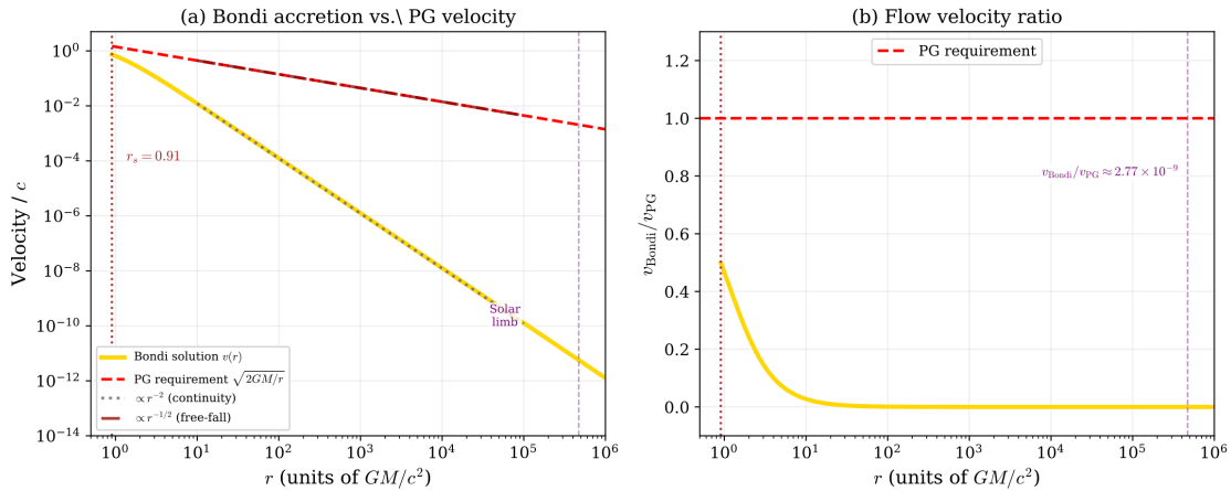
Figure 4. (a) Bondi accretion velocity (solid gold) vs. the Painlevé–Gullstrand requirement
