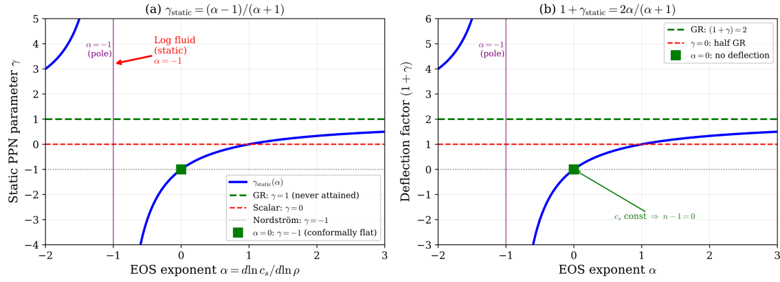
Figure 3. (a) Static PPN parameter \gamma(\alpha) = (\alpha - 1)/(\alpha + 1) . The logarithmic fluid at \bar{\rho} = \rho_\infty has \alpha = -1 , a pole of \gamma_{static} : the static acoustic metric is ill-defined. The general-relativistic value \gamma = 1 (dashed) is never attained for any finite \alpha ; it is approached only as \alpha \rightarrow \pm\infty . At \alpha = 0 the sound speed is constant, the metric is conformally flat, and \gamma = -1 , the Nordström value. (b) The deflection factor (1 + \gamma) = 2\alpha/(\alpha + 1) , which vanishes at \alpha = 0 —constant c_s , hence no refractive bending—and diverges at the pole.
