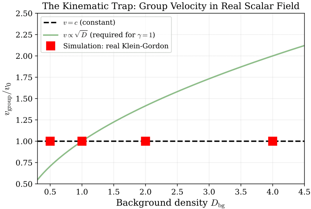
Figure 1. The kinematic trap. Group velocity of a wave packet in a Klein-Gordon field vs. background density D_{bg} . The velocity is constant (red squares), confirming Eq. (4). The green curve shows the density dependence needed for \gamma = 1 .
