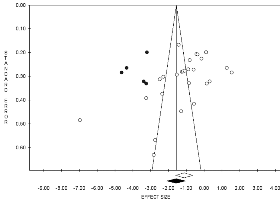
Figure 4. Funnel plot.
