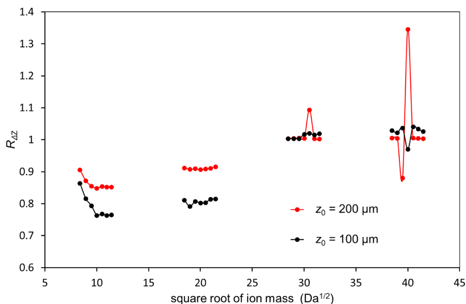
Figure 13. Variation in R_{AZ} obtained from two starting locations of ion trajectories at the same PEDDA parameter settings as Fig. 12.
