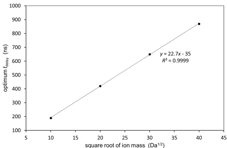
Figure 11. Linear correlation plots between square root of ion mass and the optimum t_{\text{delay}} that maximizes R_{\text{A}^{\text{TOF}}} at the fixed value of V_{\text{PEDA}} = 400 V.
