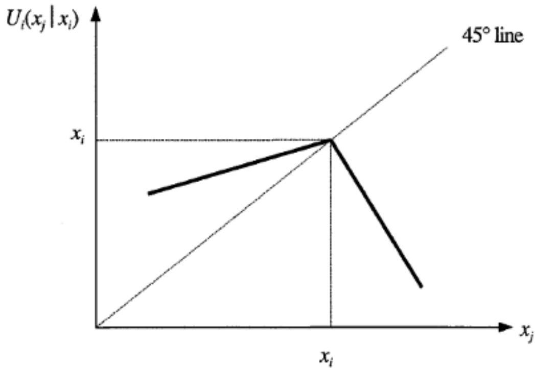
Figure 1. Utility of player i in a 2x2 game with inequity aversion (Fehr and Schmidt [1999])
