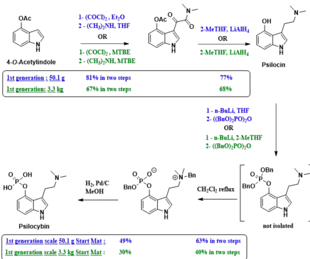
Figure 1. Sherwood's psilocin and psilocybin synthesis
